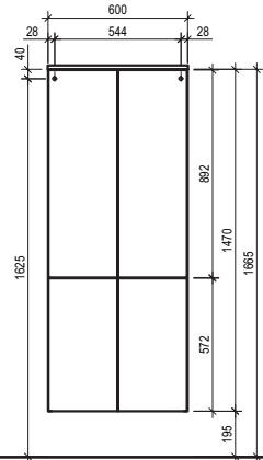
MTT6F
