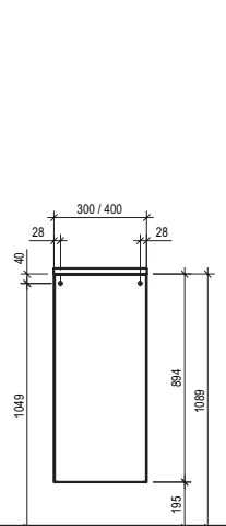
HBT4F, HBW4F
