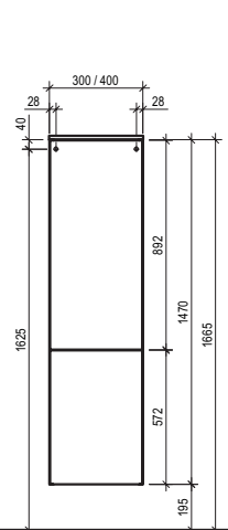
MTT4F
